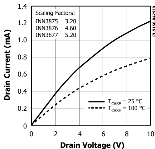
Figure 34. Output Characteristics.
