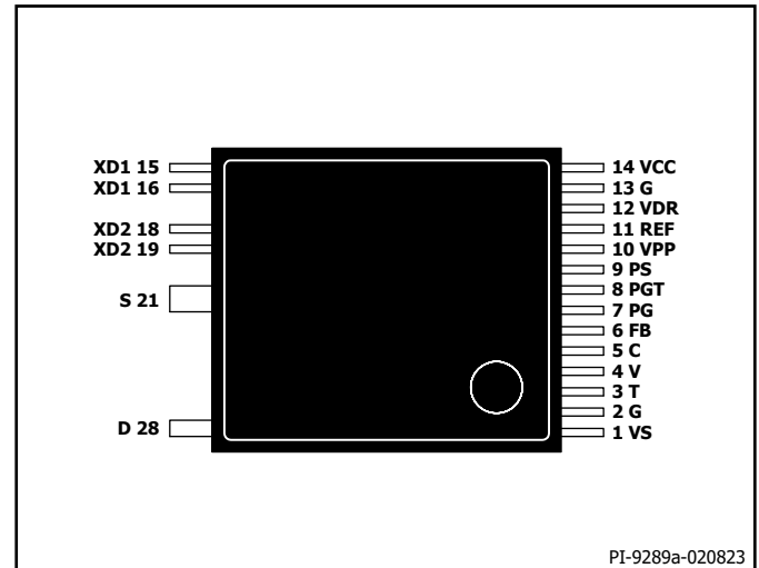
Figure 5. Pin Configuration.
