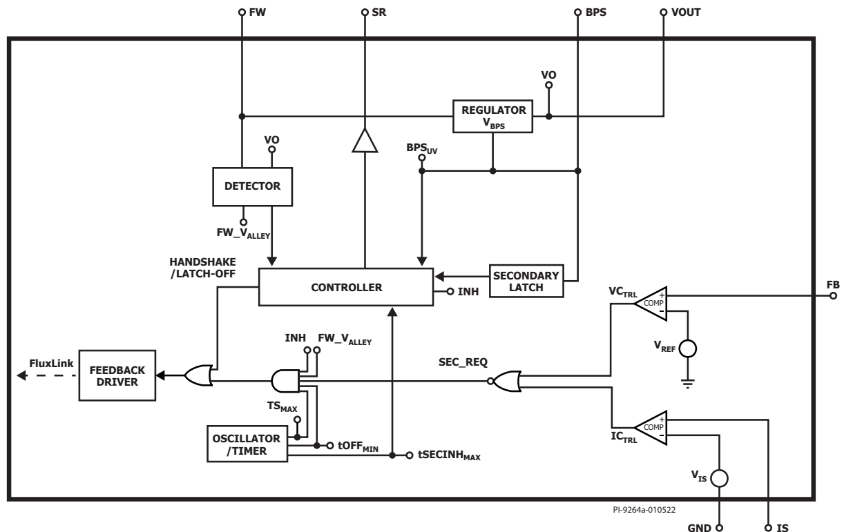
Figure 4. Secondary Controller Block Diagram.
