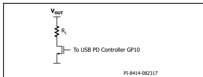
Figure 11. Active Pre-Load Circuit.
