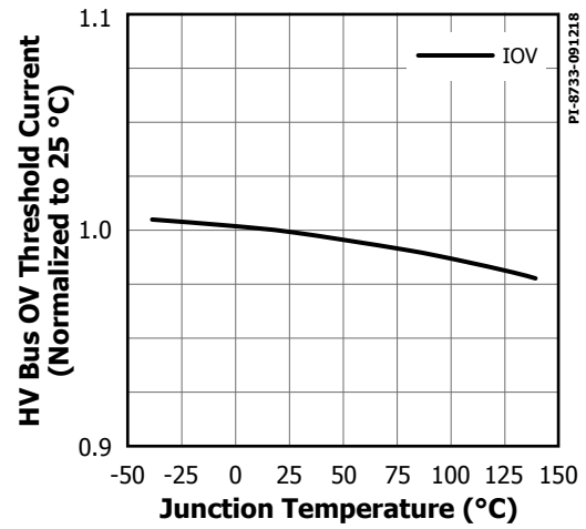
Figure 38. HV Bus OV Threshold Current vs. Temperature.
