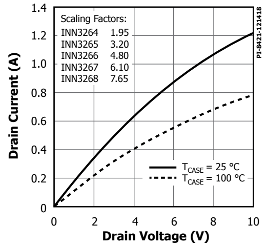
Figure 26. Output Characteristics.
