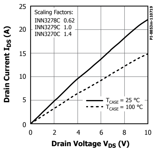
Figure 36. Output Characteristics.
