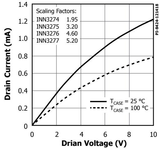
Figure 32. Output Characteristics.
