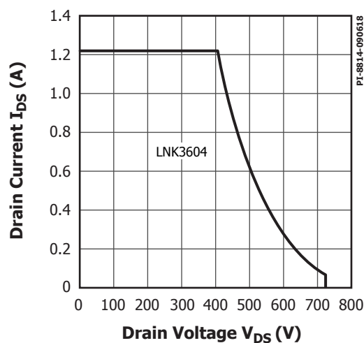
Figure 17. Maximum Allowable Drain Current vs. Drain Voltage.
