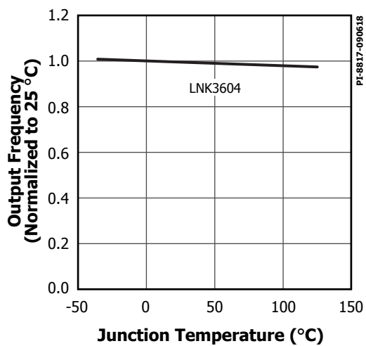
Figure 24. Output Frequency vs. Junction Temperature.
