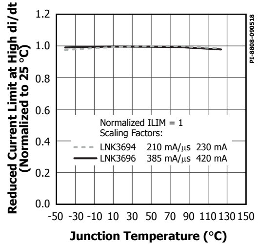
Figure 31. Reduced Current Limit vs. Junction Temperature.
