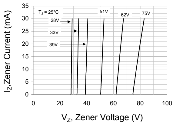
Fig.7 Typical Zener Characteristics
