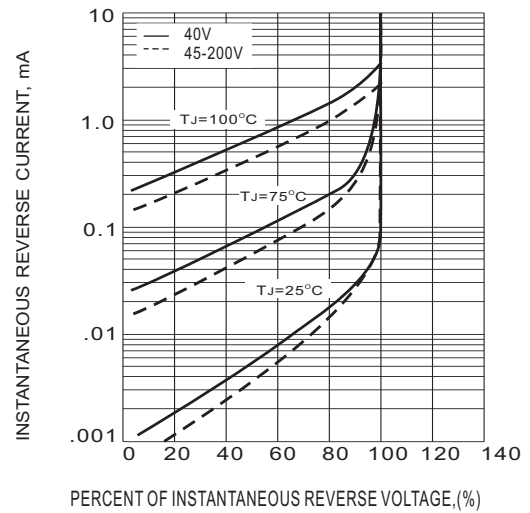
Fig.2- TYPICAL REVERSE CHARACTERISTIC
