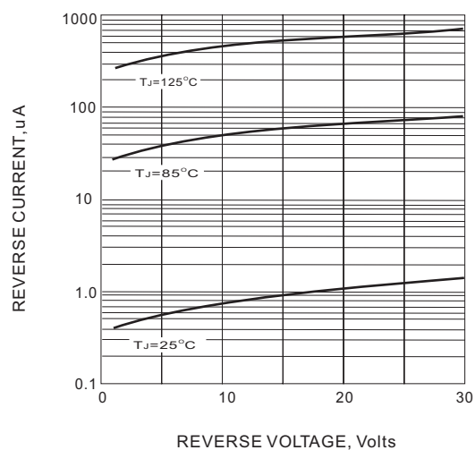
FIG. 2-TYPICAL REVERSE CHARACTERISTICS
