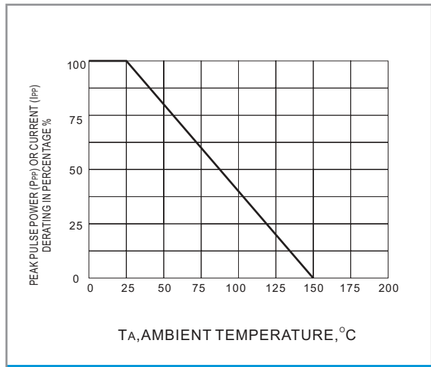
Fig.2 DERATING CURVE
