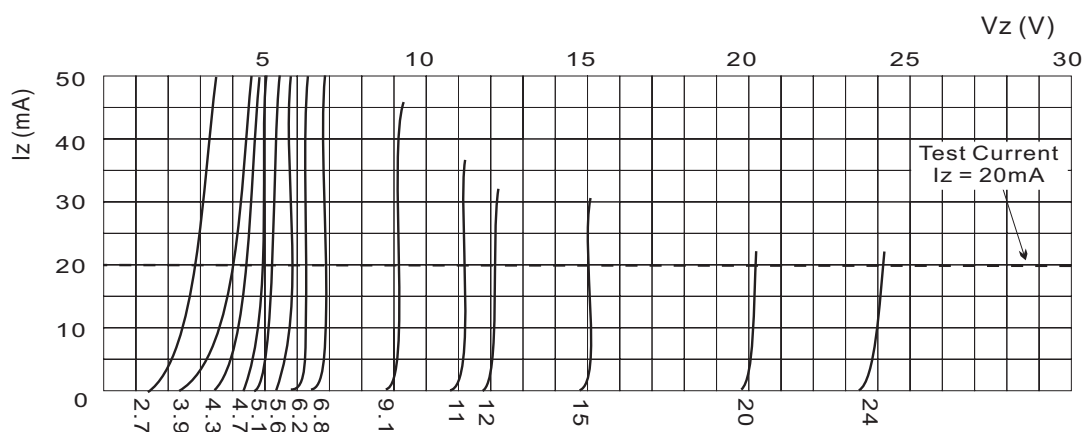
Fig.2 BREAKDOWN CHARACTERISTICS
