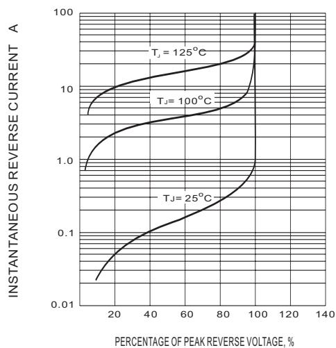
Fig.3-TYPICAL REVERSE CHARACTERISTIC
