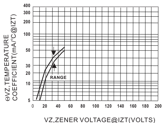
Fig.2-TEMPERATURE COEFFICIENT-RANGE
