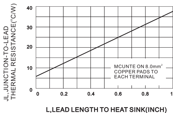
Fig.3-TYPICAL THERMAL RESISTANCE
