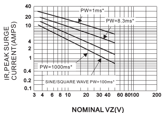
Fig.4-MAXIMUM NON-REPETITIVE SURGE CURRENT VERSUS NOMINAL ZENER VOLTAGE
