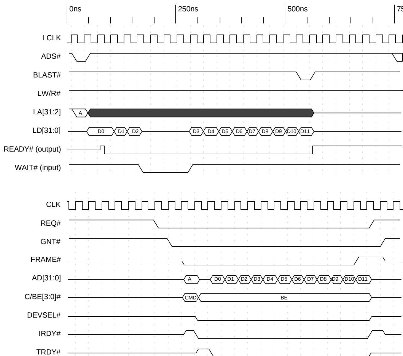
Timing Diagram 5-4. PCI Initiator Memory Write of 12 Lwords with WAIT# Input
