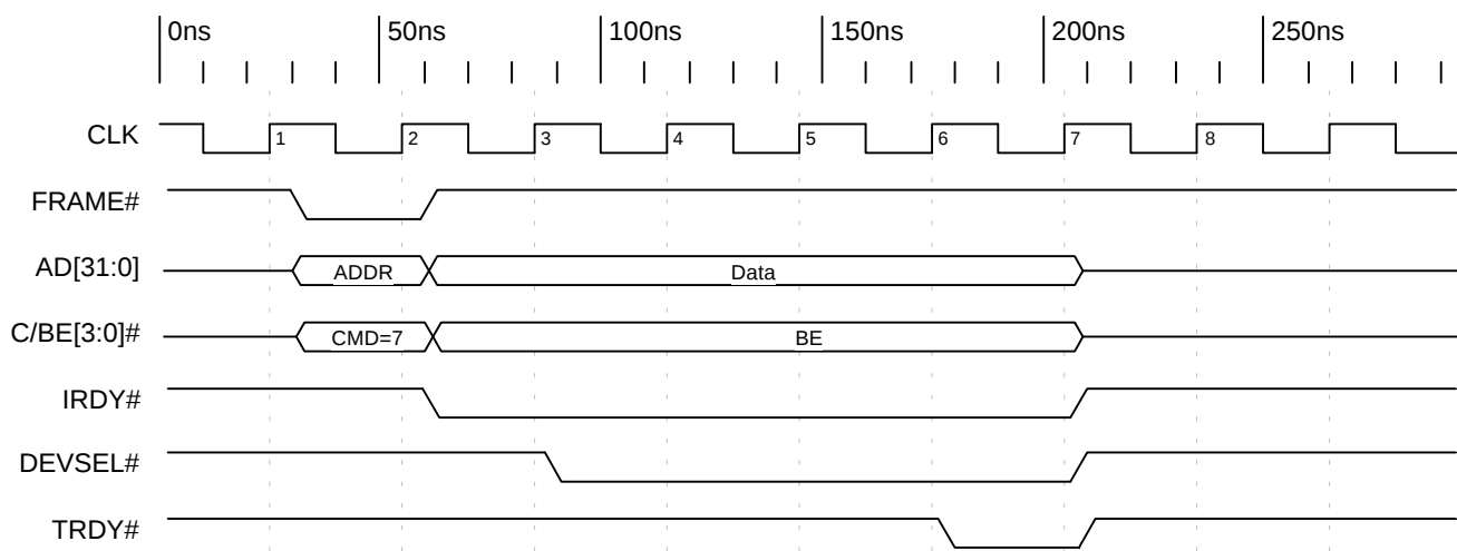
Timing Diagram 2-5. PCI Memory Write to Local Configuration Register
