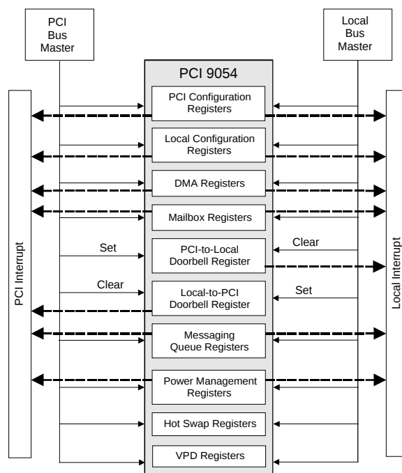
Figure 4-6. PCI 9054 Internal Register Access
