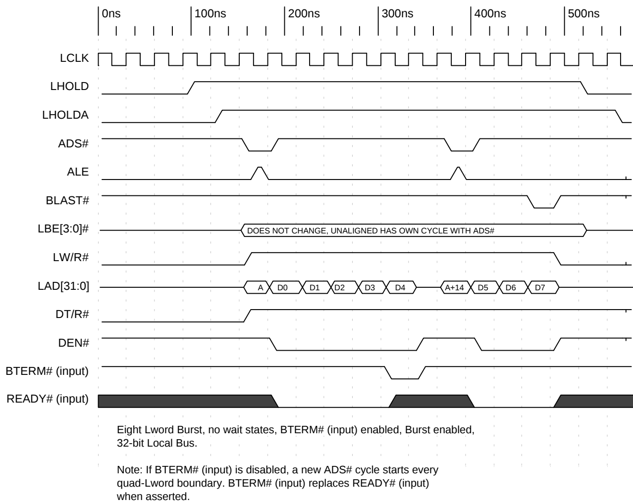
Timing Diagram 5-61. PCI Target Burst Write with Bterm Enabled (32-Bit Local Bus)
