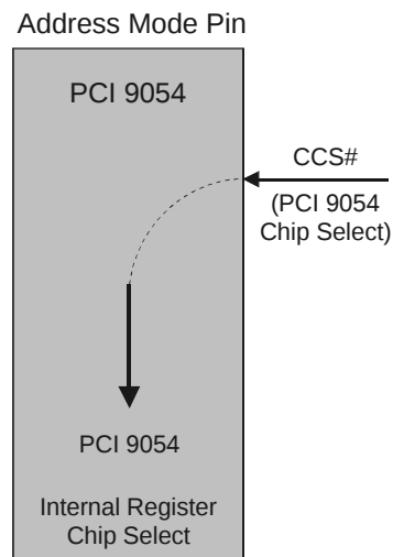
Figure 2-7. Address Decode Mode
