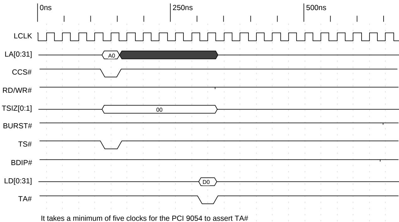
Timing Diagram 3-9. Local Configuration Read from Configuration Register
