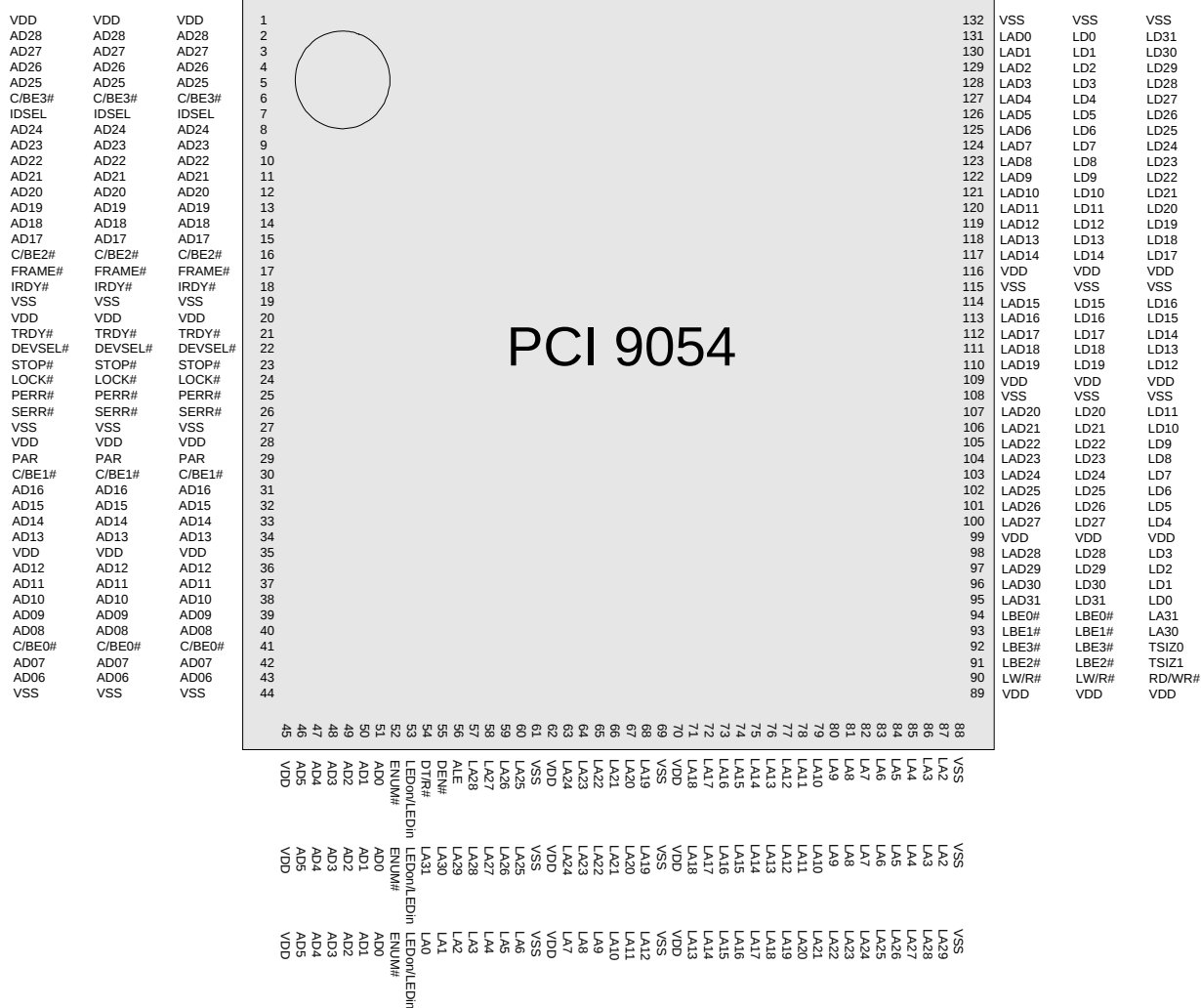
Figure 14-3. 176-Pin PQFP PCI 9054 Pinout
