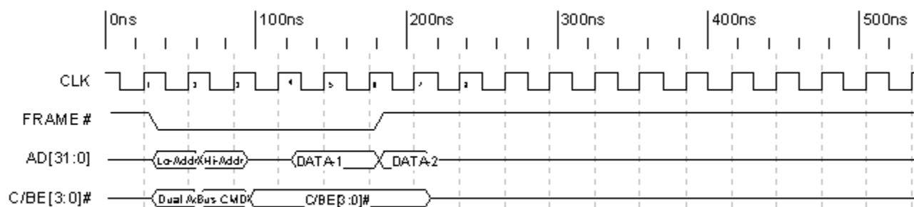
Figure 5-13. Dual Address Timing
