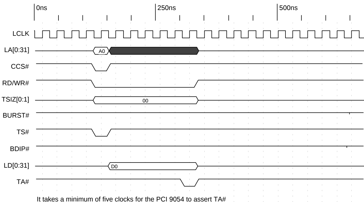
Timing Diagram 3-8. Local Configuration Write to Configuration Register
