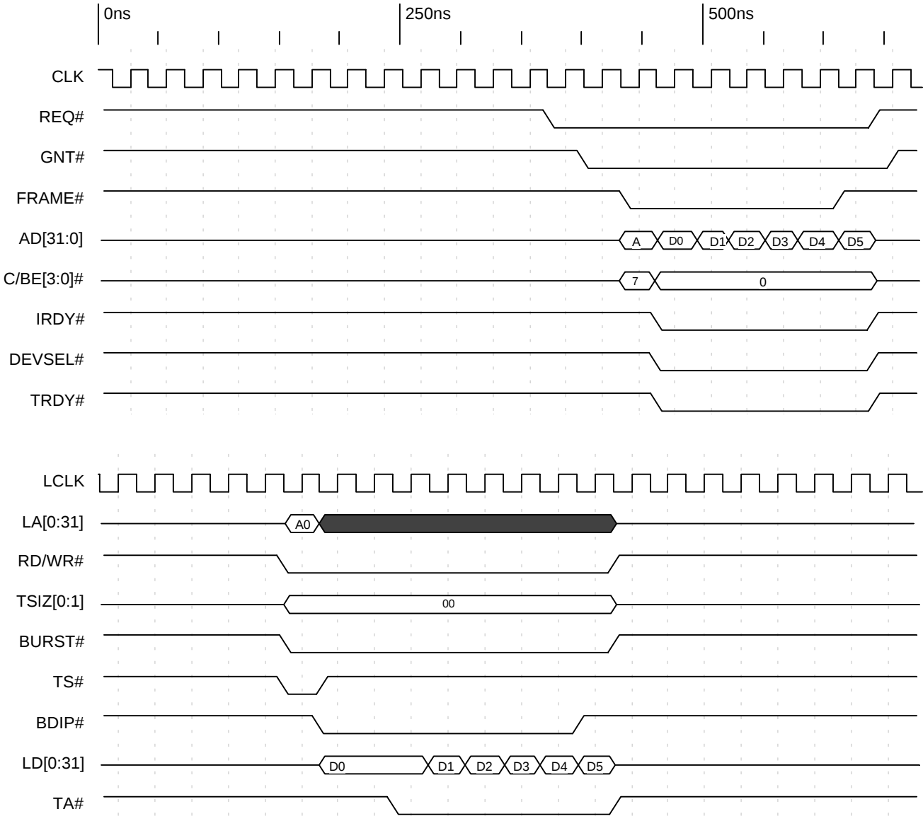
Timing Diagram 3-10. PCI Initiator Burst Write of Six Lwords beyond MPC860 Protocol
