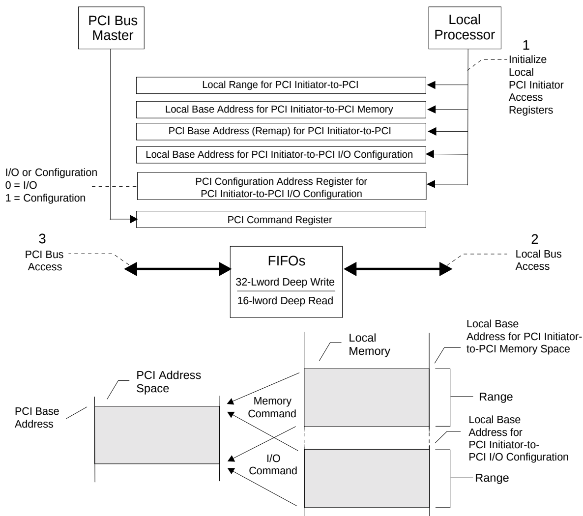
Figure 5-1. PCI Initiator Access of the PCI Bus
