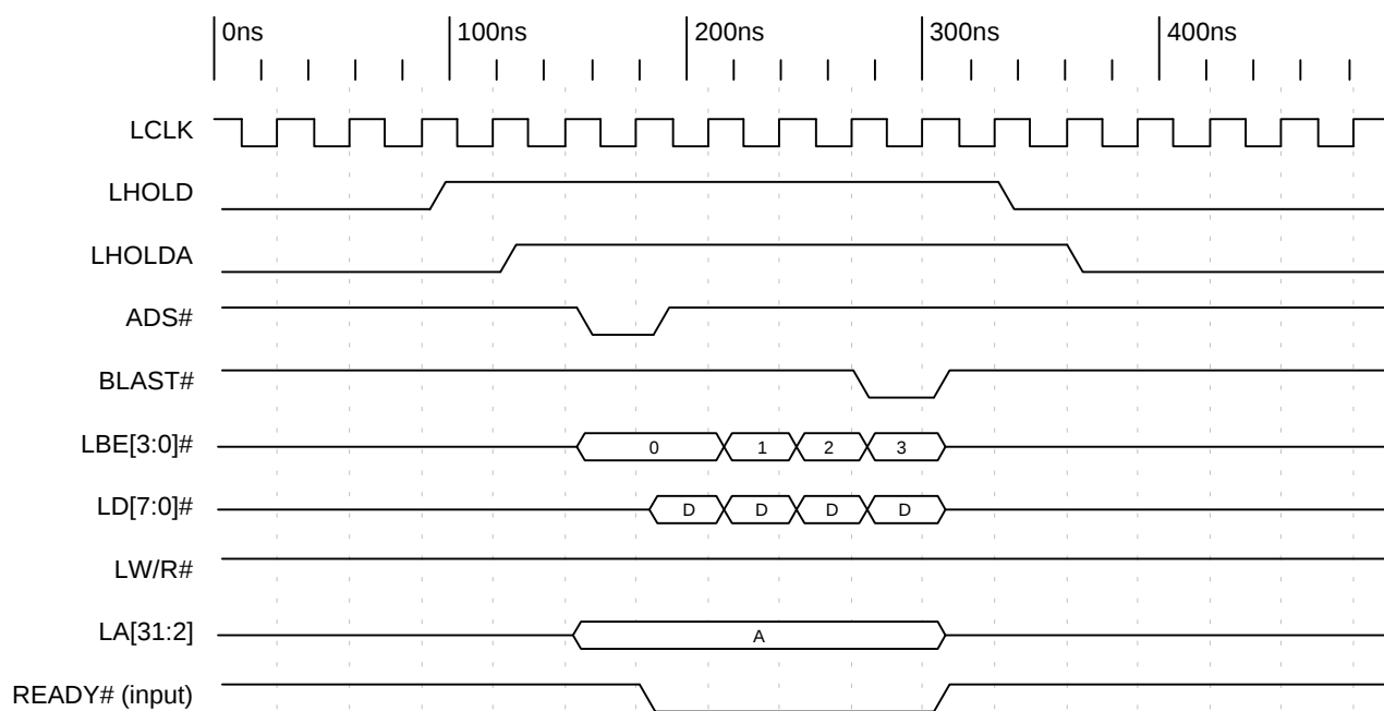
Timing Diagram 5-26. PCI Target Burst Cycle Write (8-Bit Local Bus)
