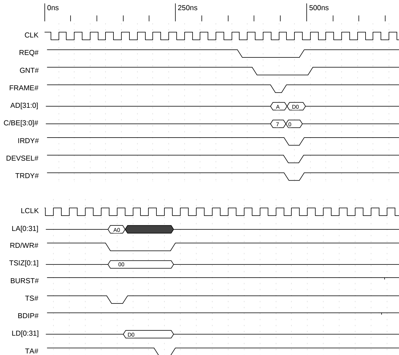
Timing Diagram 3-2. PCI Initiator Single Write Cycle, Zero Wait States
