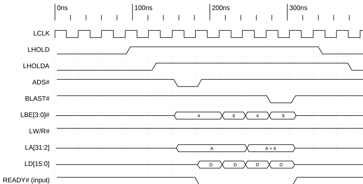
Timing Diagram 5-38. PCI Target Burst Write (16-Bit Local Bus)
