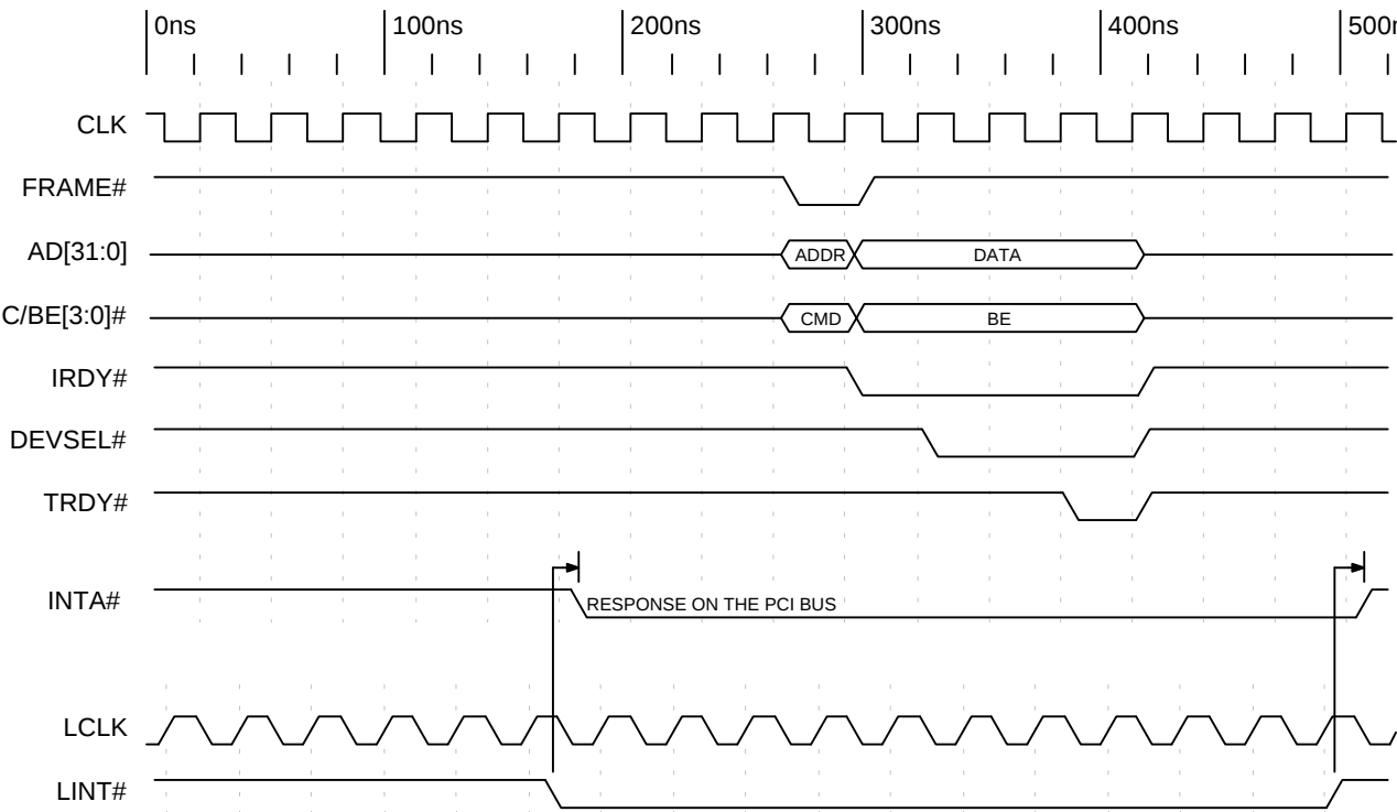
Timing Diagram 3-32. Local Interrupt Asserting PCI Interrupt
