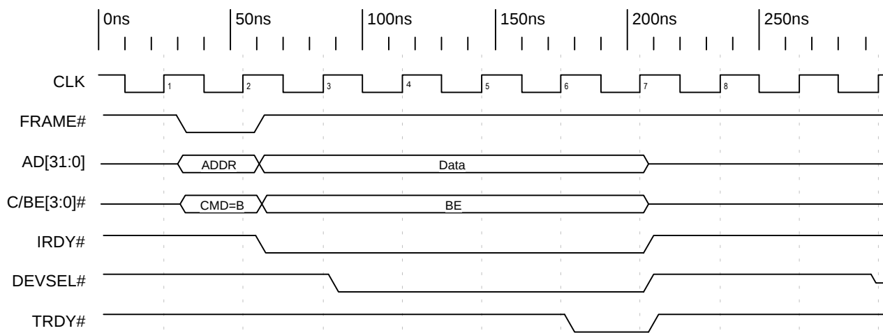
Timing Diagram 5-19. PCI Configuration Write to PCI Configuration Register
