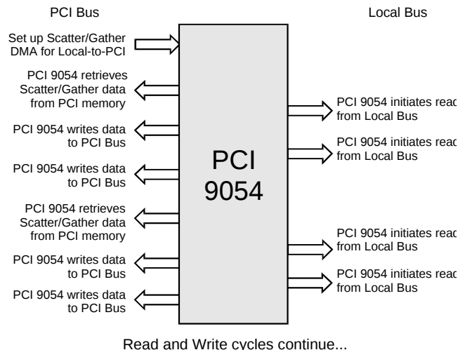
Figure 5-15. Scatter/Gather DMA Mode from Local-to-PCI Bus (Control Access from the PCI Bus)
