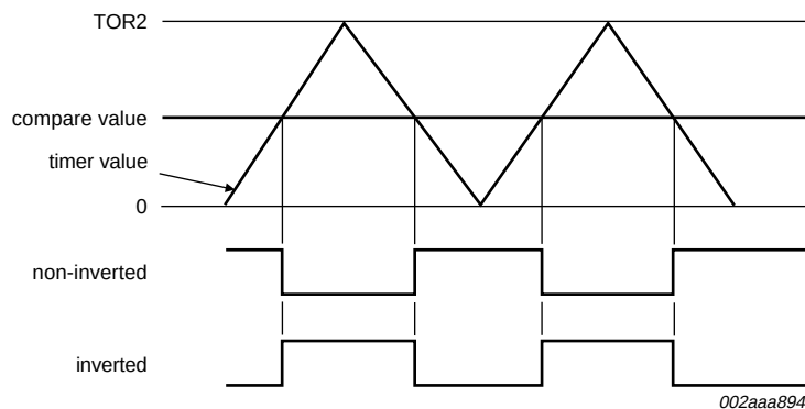
Fig 9. Symmetrical PWM.
