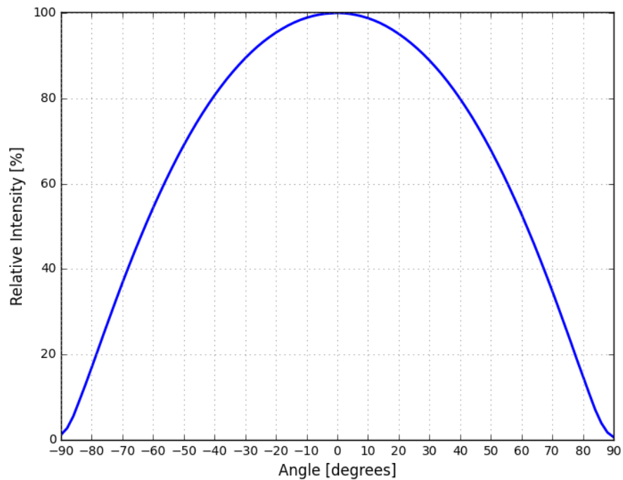
Figure 10. Typical radiation pattern for LUXEON Altilon SMD-A 1x4
