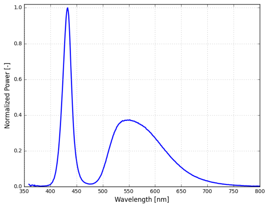
Figure 2. Typical normalized power vs. wavelength for LUXEON Altilon SMD-A 1x4 at MP binning condition
