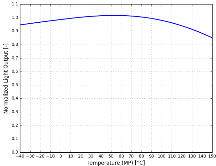
Figure 3. Typical normalized light output vs. temperature for LUXEON Altilon SMD-A 1x4 at MP binning current
