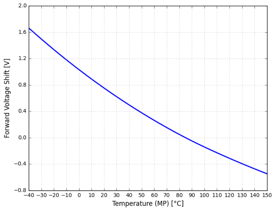
Figure 6. Typical forward voltage shift vs. temperature for LUXEON Altilon SMD-A 1x4 at MP binning current
