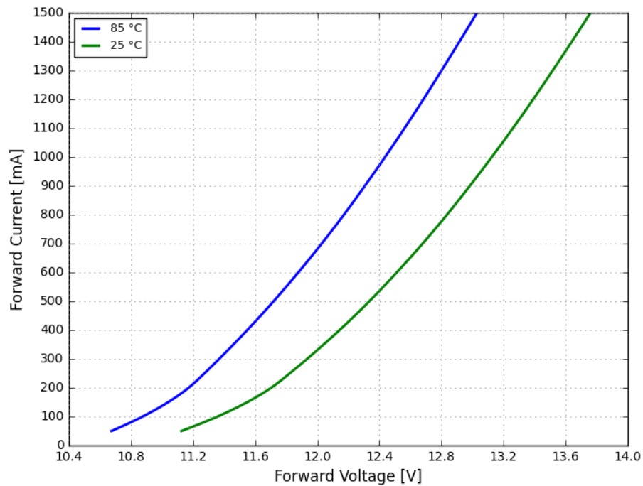
Figure 5. Typical forward current vs. forward voltage for LUXEON Altilon SMD-A 1x4 at MP binning temperature and at room temperature
