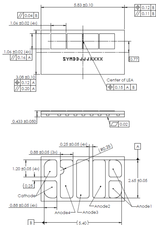
Figure 14. Mechanical dimensions for LUXEON Altilon SMD-A 1x4
