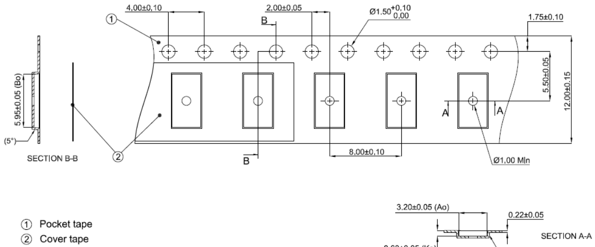
Figure 15. Pocket tape dimensions for LUXEON Altilon SMD-A 1x4
