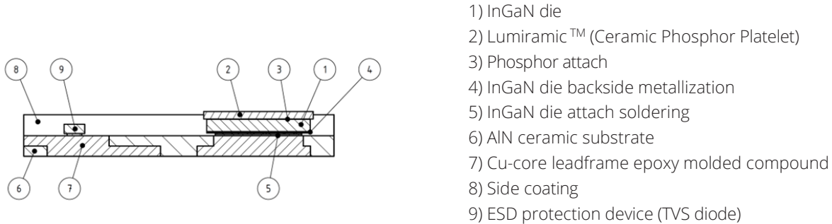
Figure 1. Schematic cross section LUXEON Altilon SMD-A 1x4
