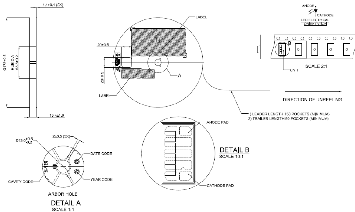
Figure 16. Reel dimensions for LUXEON Altilon SMD-A 1x4
