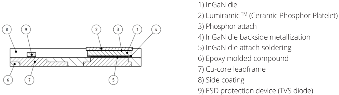
Figure 1. Schematic cross section LUXEON Altilon SMD-A 1x3
