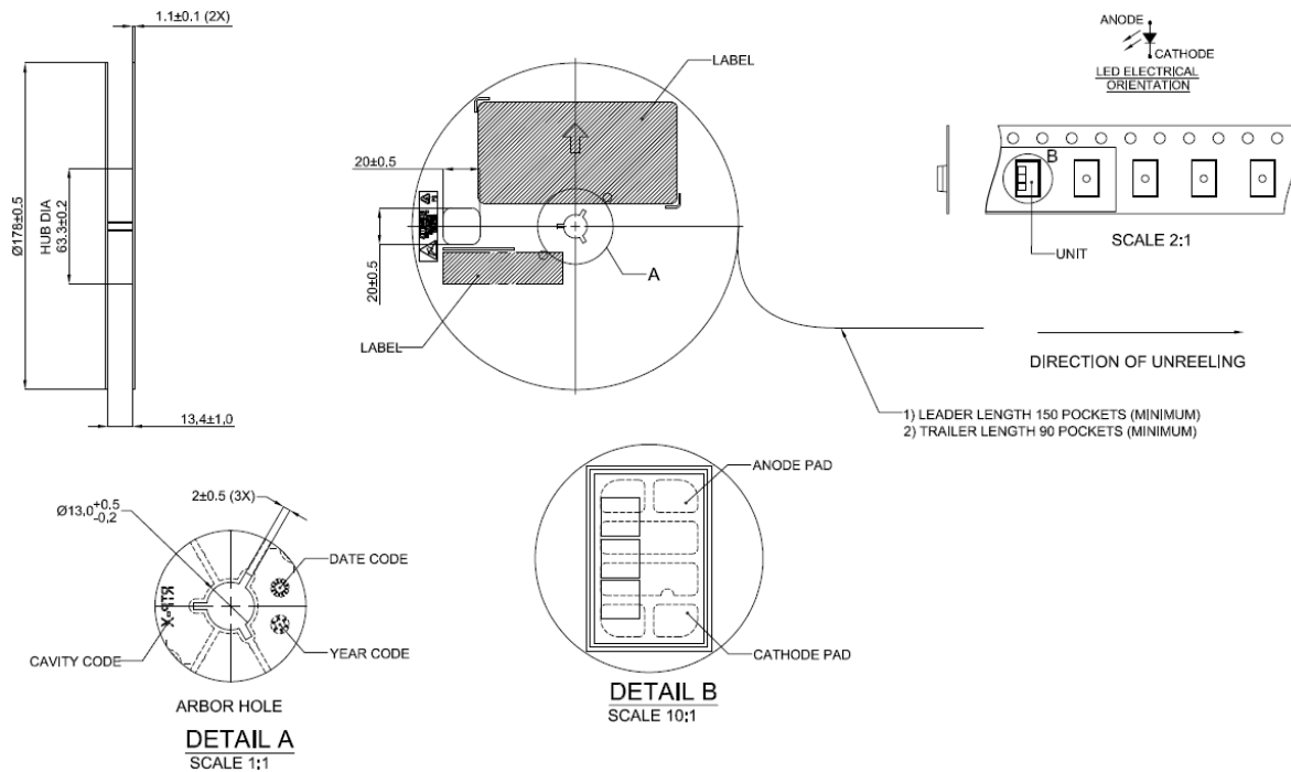
Figure 16. Reel dimensions for LUXEON Altilon SMD-A 1x3
