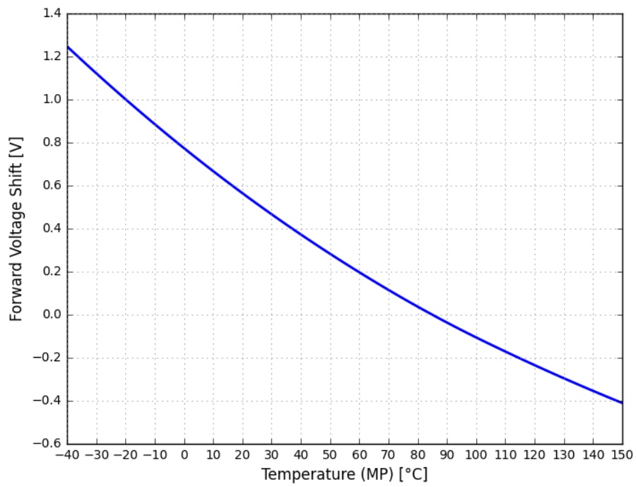
Figure 6. Typical forward voltage shift vs. temperature for LUXEON Altilon SMD-A 1x3 at MP binning current
