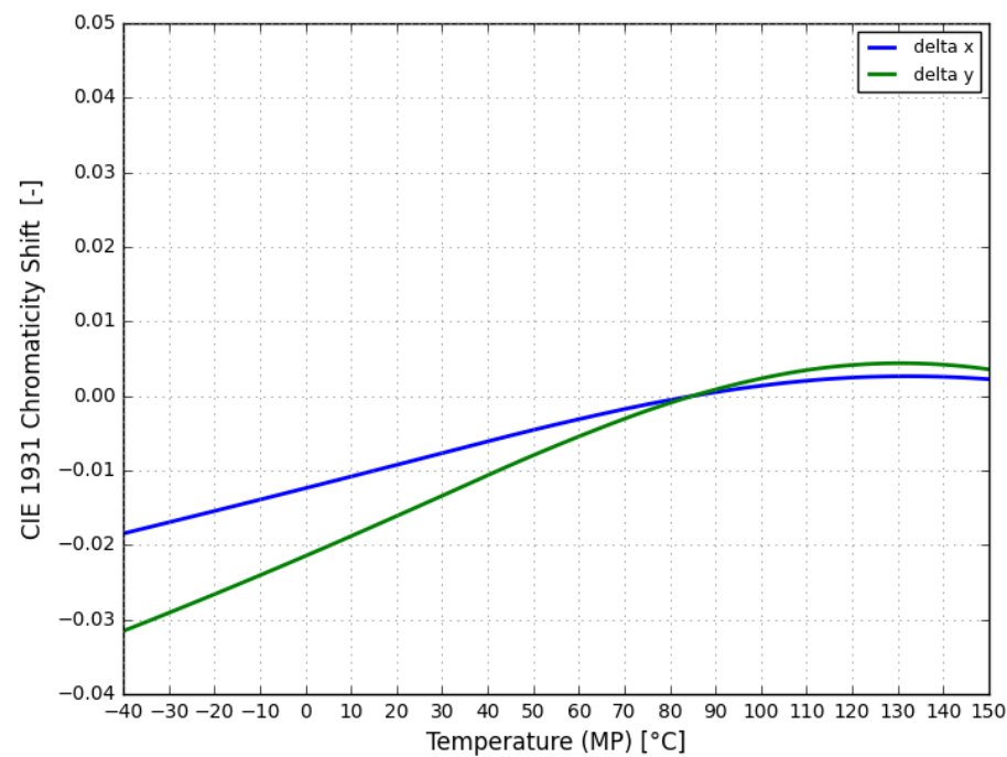
Figure 7. Typical color shift in CIE1931 x, y coordinates vs. temperature for LUXEON Altilon SMD-A 1x3 at MP binning current
