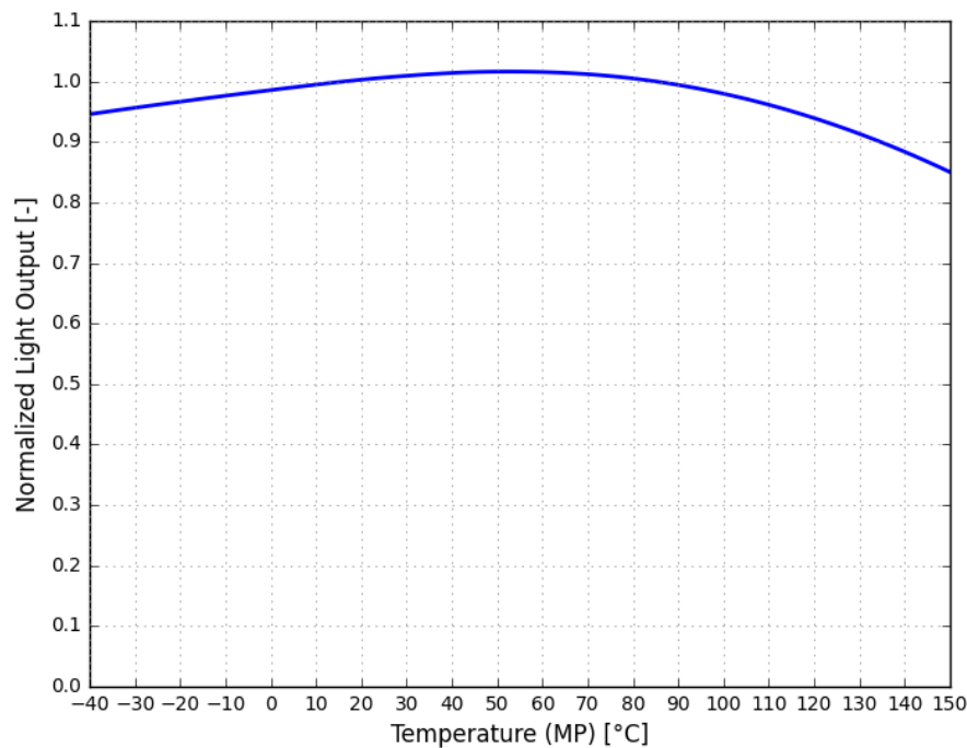
Figure 3. Typical normalized light output vs. temperature for LUXEON Altilon SMD-A 1x3 at MP binning current
