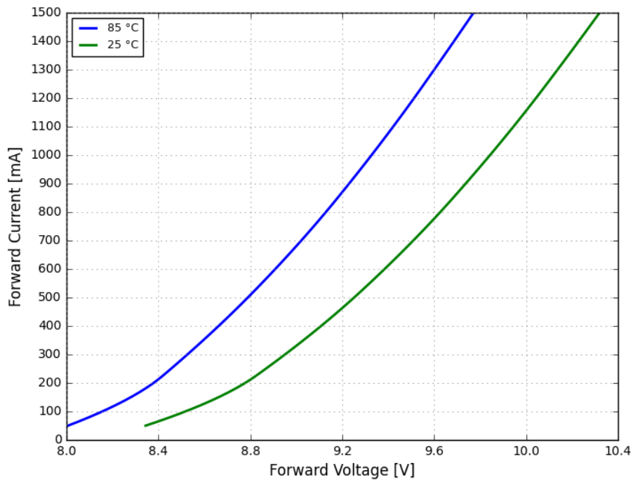
Figure 5. Typical forward current vs. forward voltage for LUXEON Altilon SMD-A 1x3 at MP binning temperature and at room temperature
