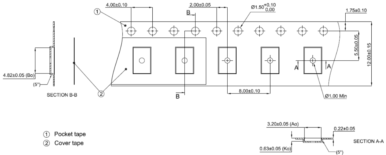
Figure 15. Pocket tape dimensions for LUXEON Altilon SMD-A 1x3
