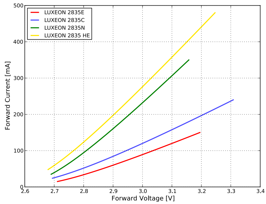
Figure 4c. Typical forward current vs. forward voltage for LUXEON 2835C Line 3V at T j =25°C.
