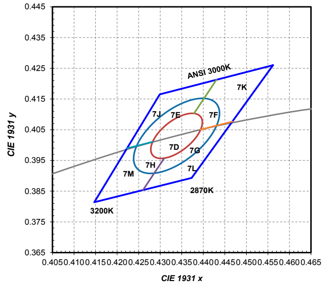
Figure 8c. 1/9 th color bin structure for LUXEON 2835E and LUXEON 2835C 3000K at specified test current and binning temperatures of T_j=25^{\circ}\text{C} and T_j=85^{\circ}\text{C} .
