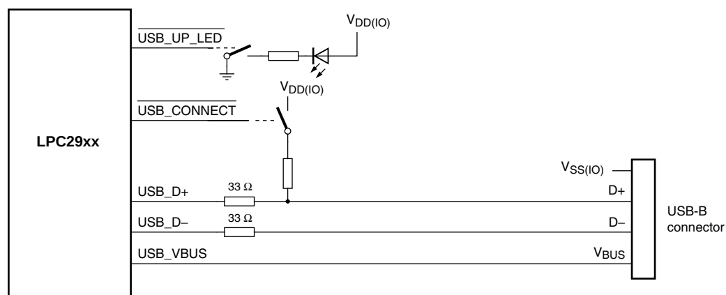
Fig 35. LPC2926/2927/2929 USB device port configuration
