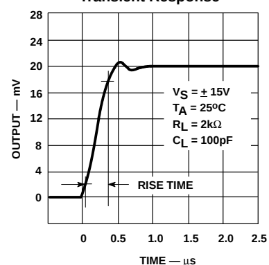
Transient Response
