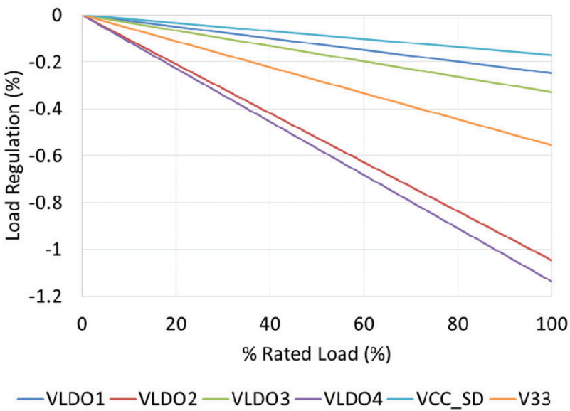
Figure 26. Load regulation - LDOs
