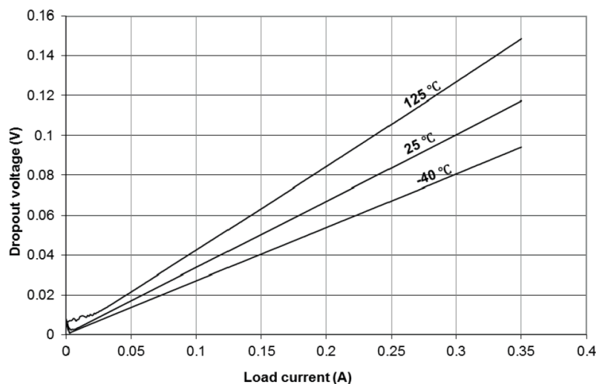
Figure 31. Dropout voltage - VLDO4, V33 - V OUT = 3.3 V
