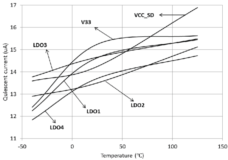
Figure 24. Quiescent current - LDOs
