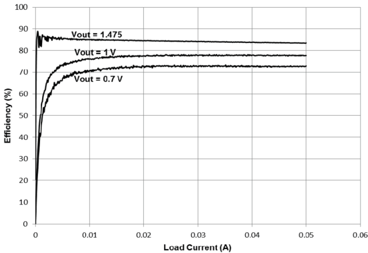
Figure 28. SW1A efficiency - PFM mode
