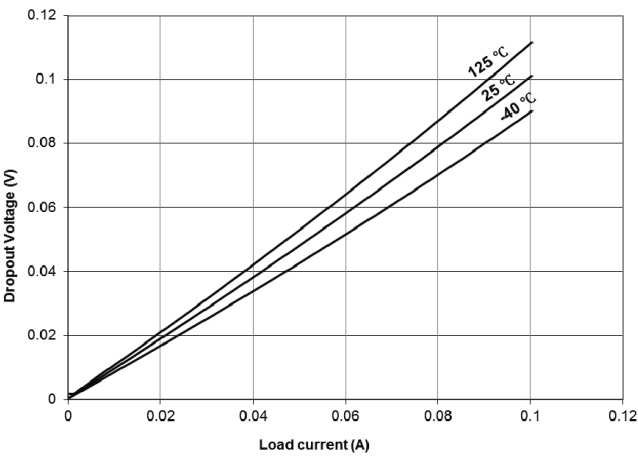
Figure 30. Dropout voltage - VLDO1, VLDO3, VCC_SD - V OUT = 1.8 V
