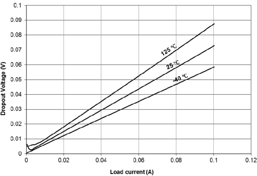
Figure 29. Dropout voltage - VLDO1, VLDO3, VCC_SD - V OUT = 3.3 V
