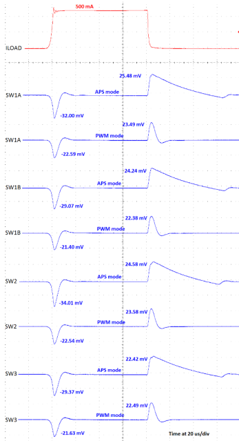
Figure 19. Load transient response - buck regulators
