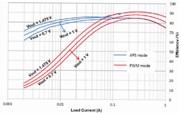
Figure 27. SW1A efficiency - APS and PWM modes
