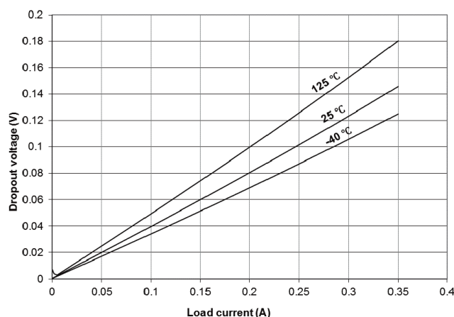
Figure 32. Dropout voltage - VLDO4 - V OUT = 1.8 V
