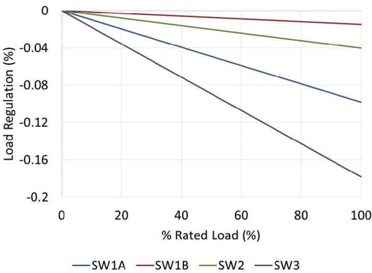
Figure 25. Load regulation - buck regulators
