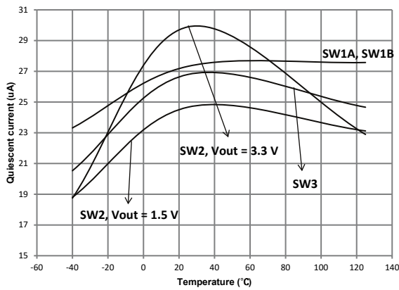
Figure 23. Quiescent current - buck regulators in PFM mode
