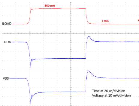
Figure 18. Load transient response - LDO4 and V33
