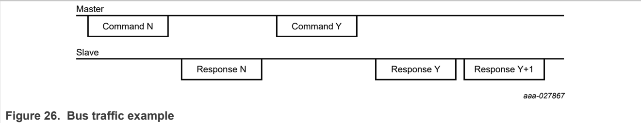
Figure 26. Bus traffic example
