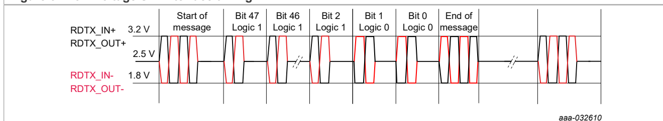
Figure 6. Transformer communication signaling
