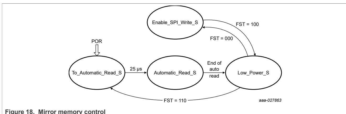
Figure 18. Mirror memory control
