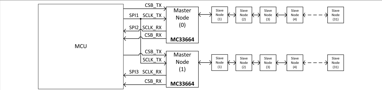
Figure 36. Example of multiple daisy chain.
