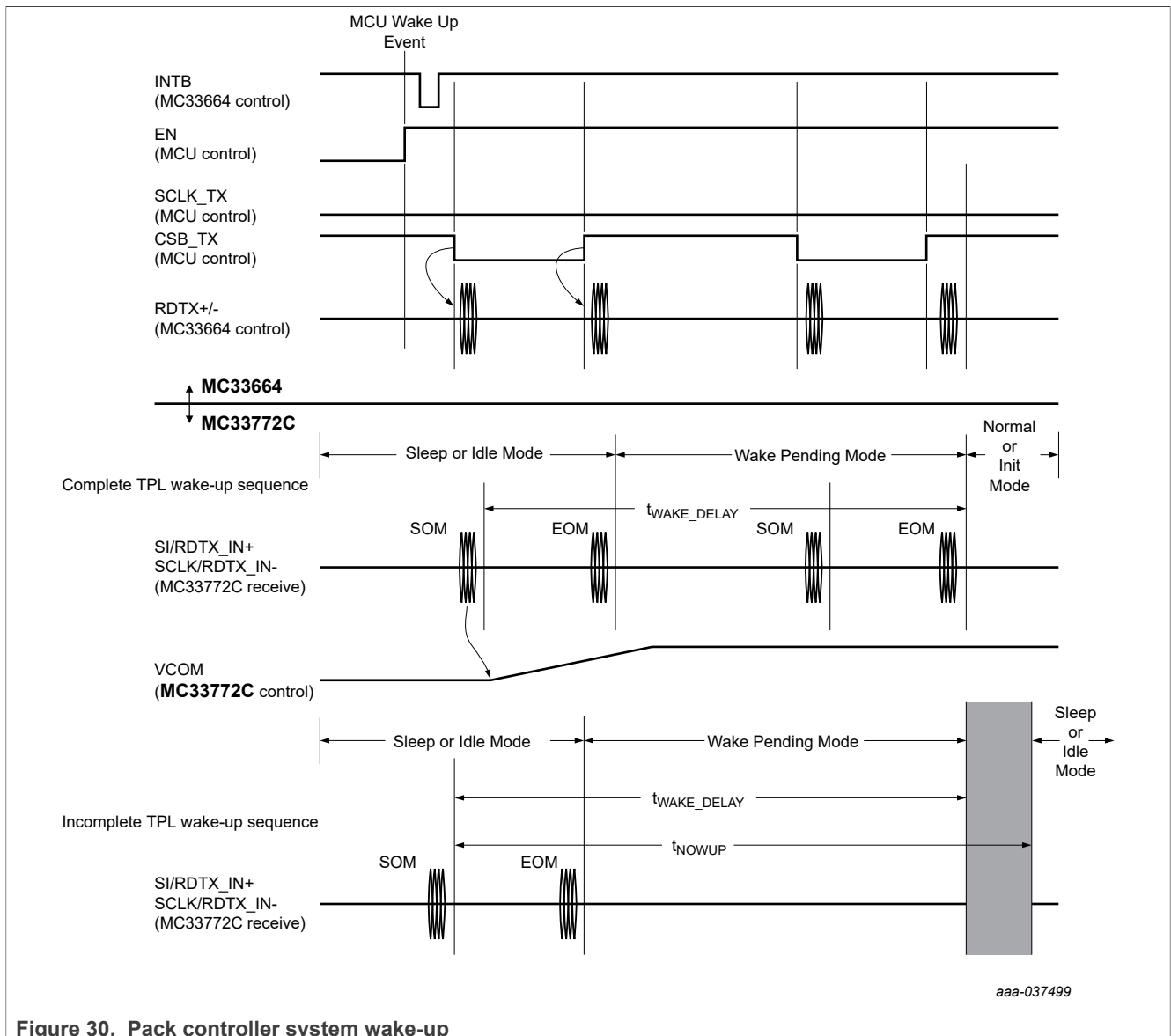
Figure 30. Pack controller system wake-up
