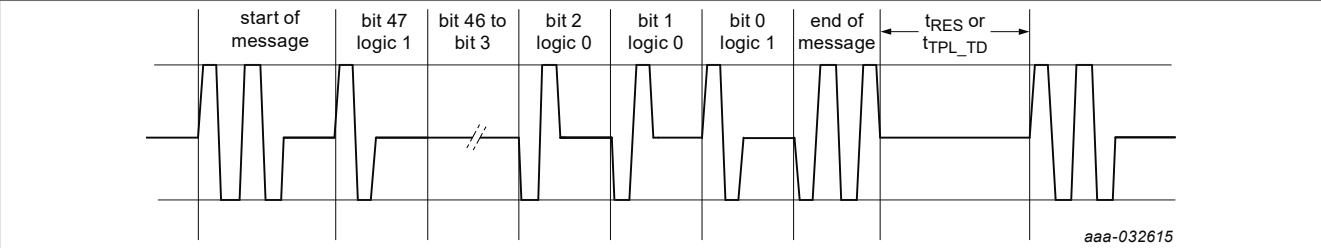
Figure 28. Transformer communication waveforms
