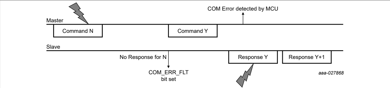
Figure 27. Bus traffic with receive error and recovery
