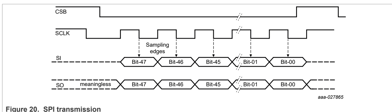
Figure 20. SPI transmission
