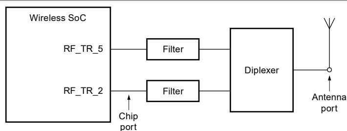
Figure 14. RF performance measurement points
