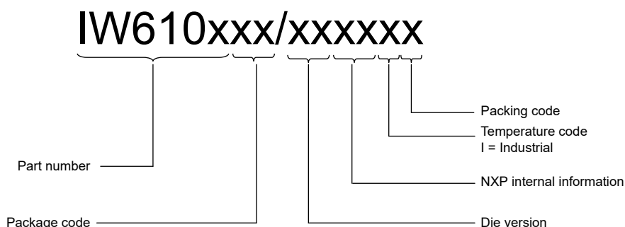
Figure 6. Part numbering scheme
