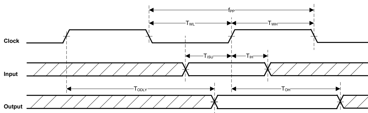
Figure 16. SDIO protocol timing diagram—High-speed mode
