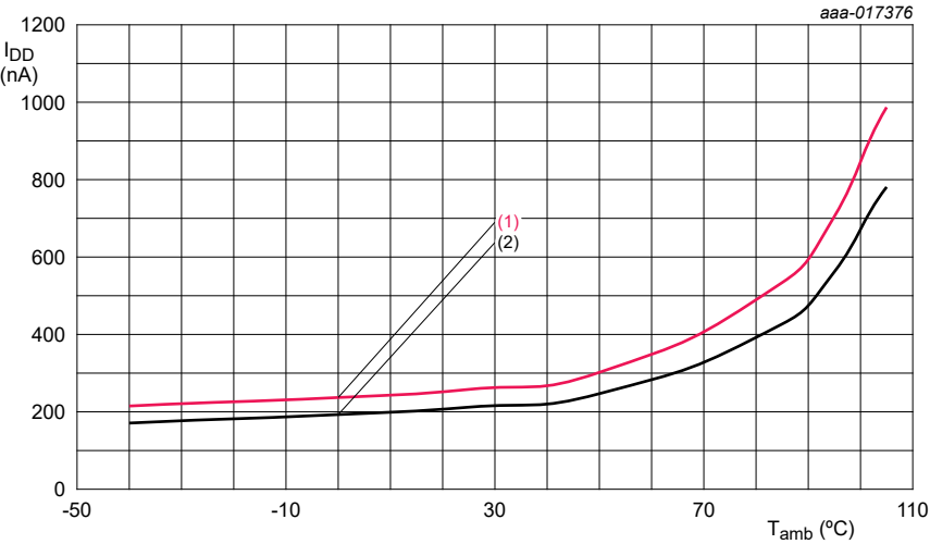
C L(itg) = 7 pF; CLKOUT disabled. 1. V DD = 5.5 V. 2. V DD = 3.3 V.
