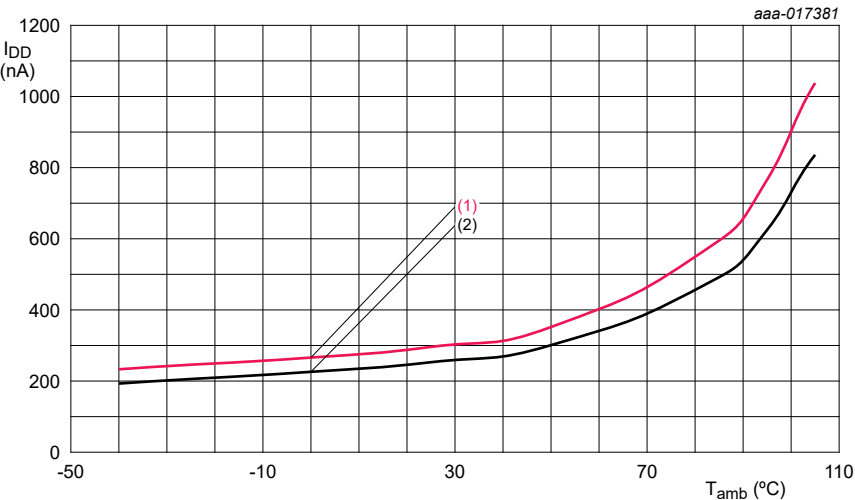
C L(itg) = 12.5 pF; CLKOUT disabled. 1. V DD = 5.5 V. 2. V DD = 3.3 V.
