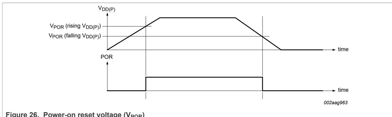
Figure 26. Power-on reset voltage ( V_{POR} )
