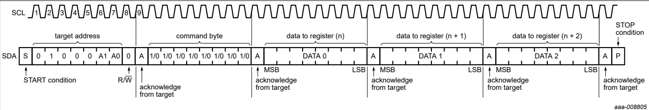
Figure 16. Write to device registers (operate as register triples)
