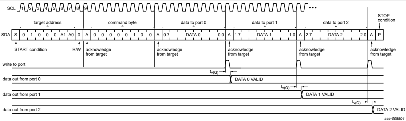
Figure 15. Write to output port register
