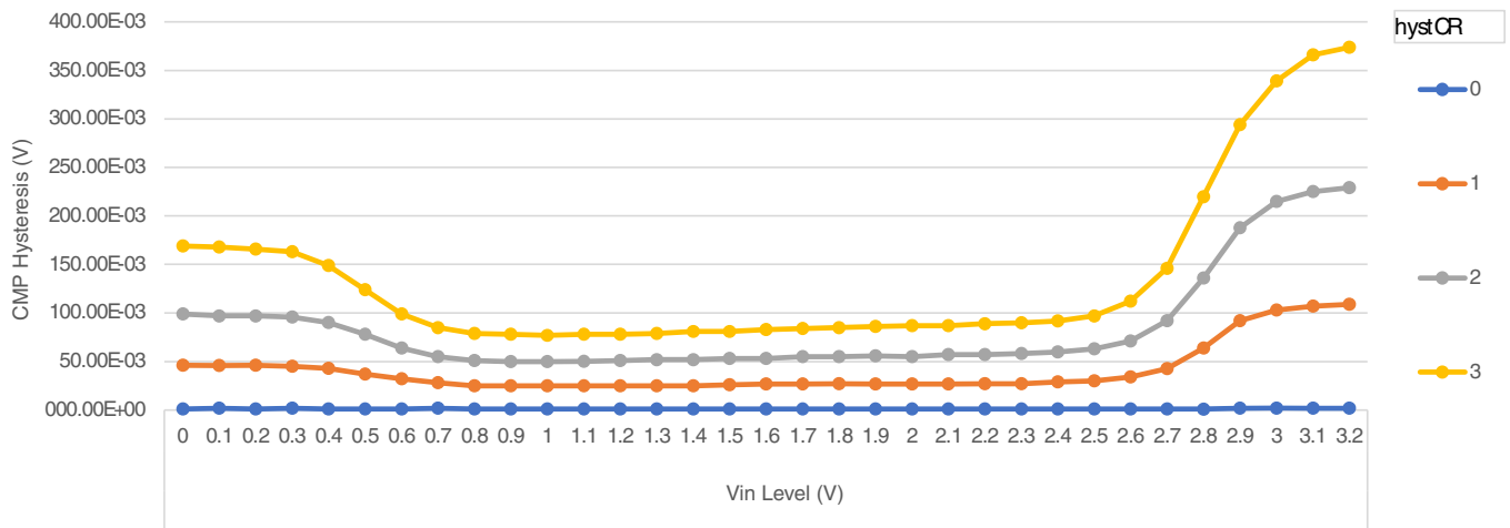
Figure 12. Typical hysteresis vs. Vin level ( V_{DD} = 3.3 \text{ V} , \text{PMODE} = 1 )
