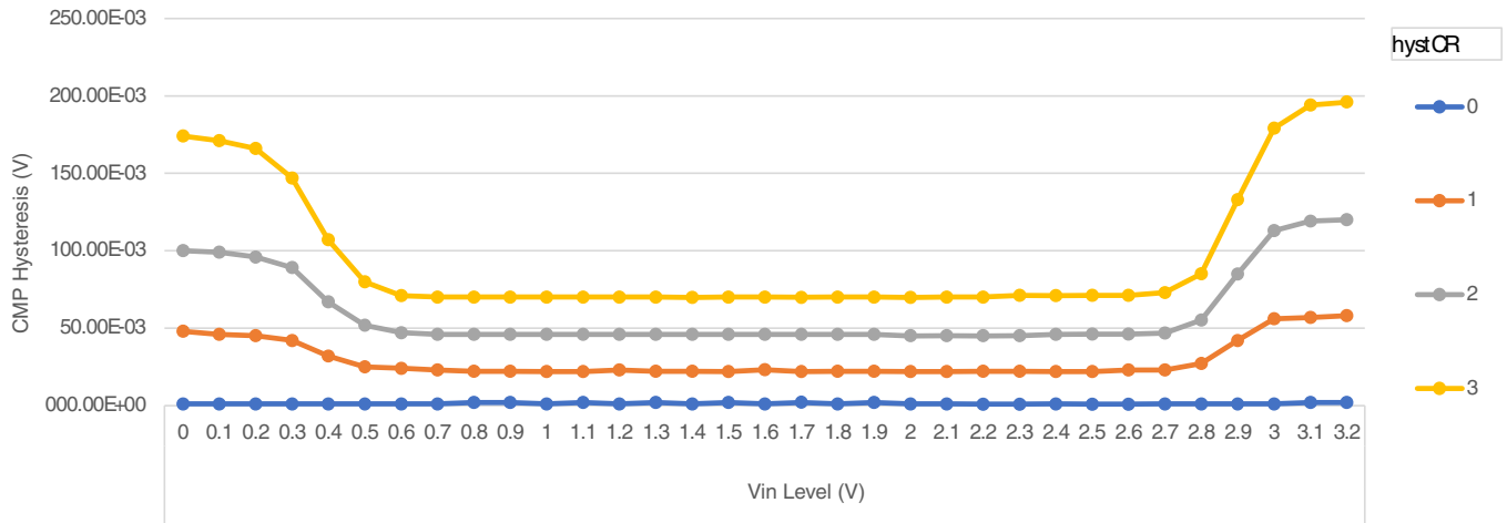
Figure 11. Typical hysteresis vs. Vin level ( V_{DD} = 3.3 \text{ V} , \text{PMODE} = 0 )
