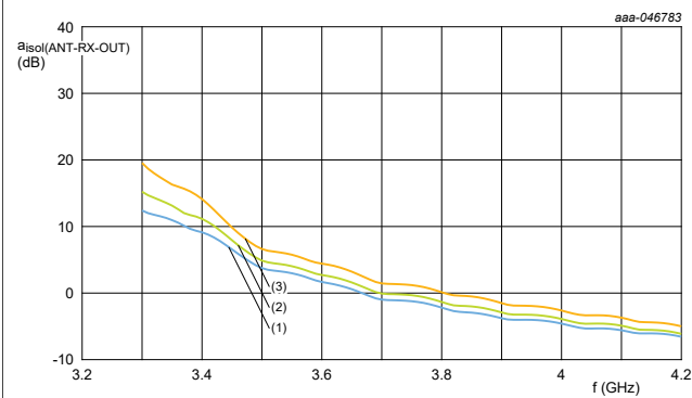
Figure 23. High gain Loopback mode, ANT to RX_OUT isolation versus frequency over temperature
