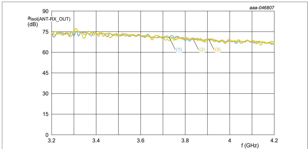
Figure 25. Isolation mode ANT to RX_OUT versus frequency over temperature
