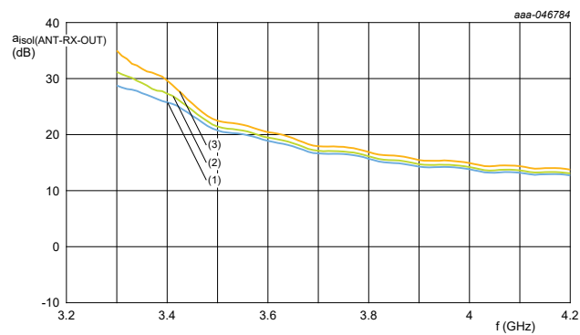
Figure 24. Low gain Loopback mode, ANT to RX_OUT isolation versus frequency over temperature
