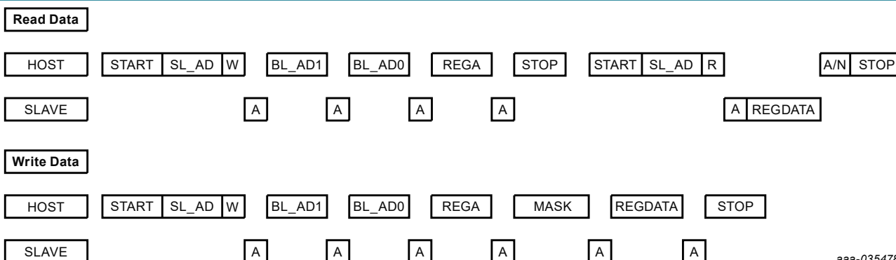
Figure 11. READ REGISTER and WRITE REGISTER command
