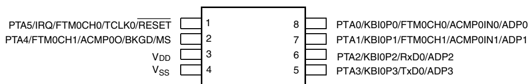
Figure 17. 8-pin SOIC package
