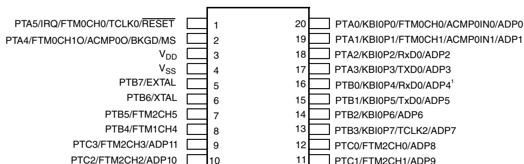
Figure 15. 20-pin TSSOP package
