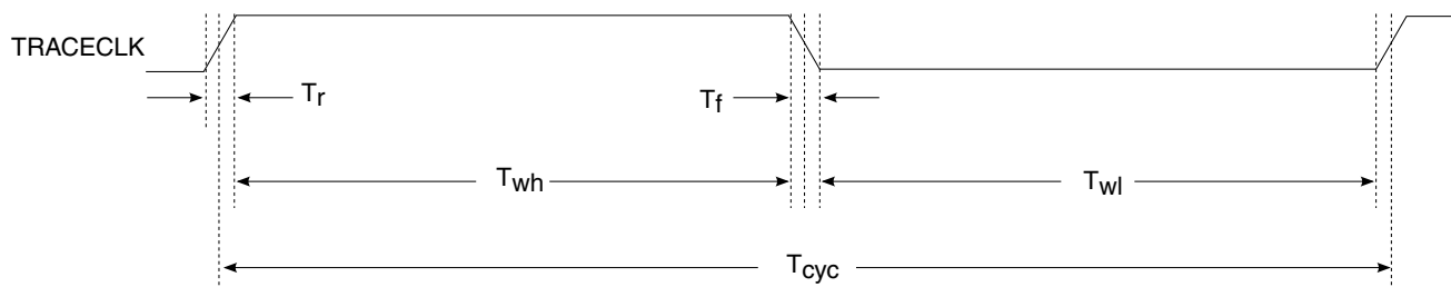
Figure 9. TRACE_CLKOUT specifications
