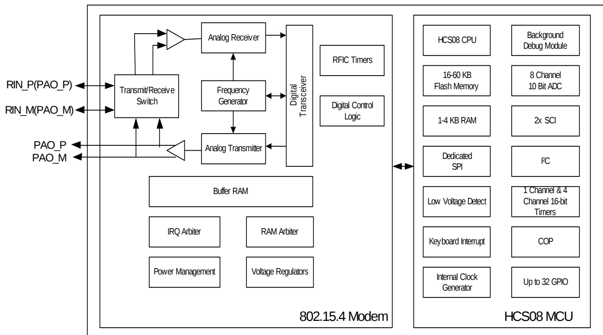
Figure 1. MC1321x System Level Block Diagram
