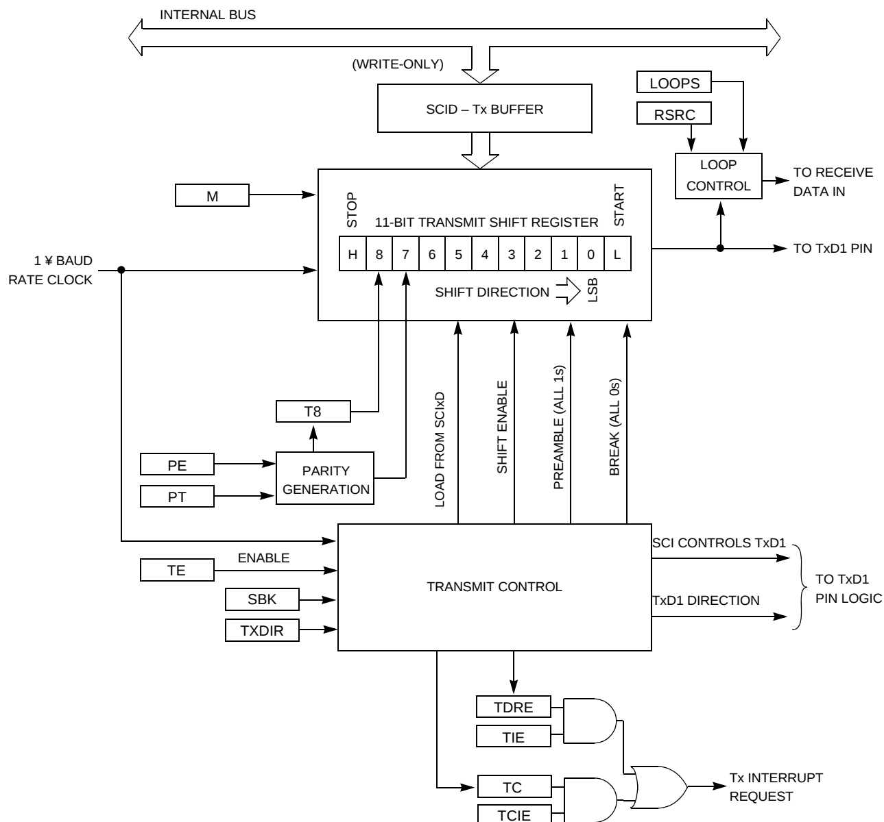
Figure 22. SCI Transmitter
