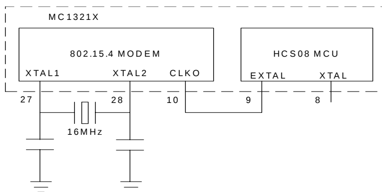
Figure 2. MC1321x Single Crystal System Clock Structure
