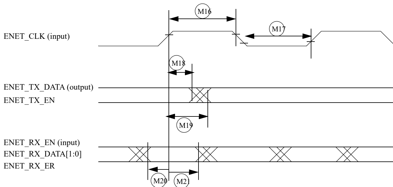
Figure 16. RMI mode signal timing diagram
