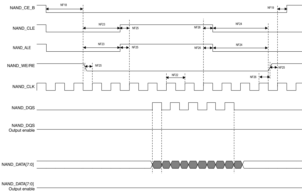
Figure 27. Source Synchronous mode data read timing diagram
