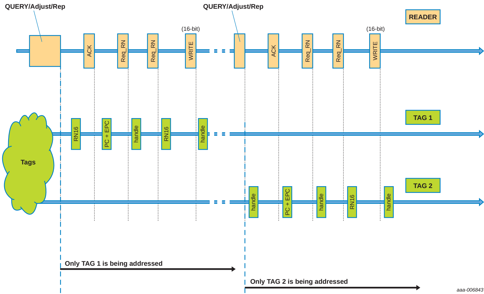
Fig 7. Example of 16-bit Write command with standard EPC Gen 2 commands
