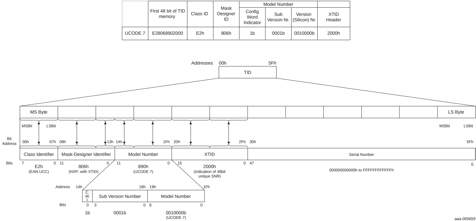
Fig 6. UCODE 7 TID memory structure
