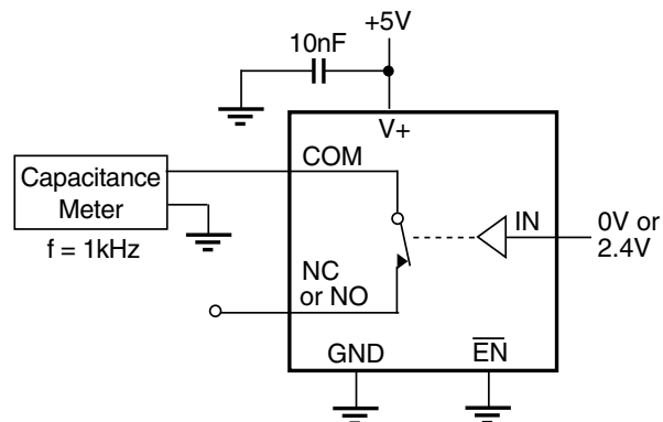
Figure 6. Channel-On Capacitance
