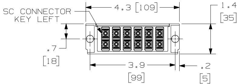
FRONT VIEW SHOWN W/O DUSTCAPS
