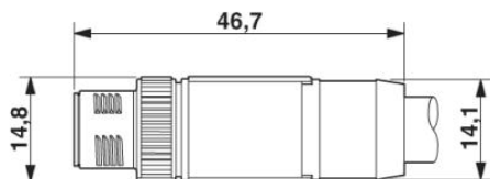
M12 SPEEDCON plug, straight, shielded
