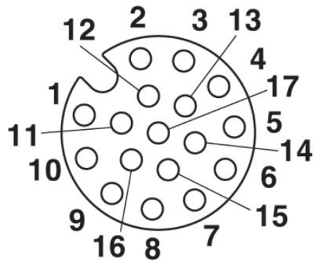
Pin assignment M12, 17-pos., socket side view
