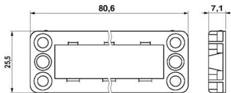
Panel mounting frame dimensional drawing
