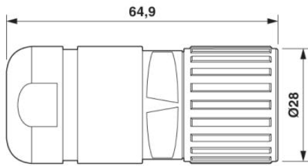
Dimensioned drawing
