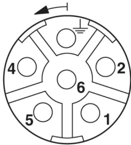
Schematic diagram
