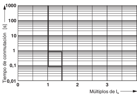
Trigger characteristic
