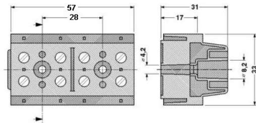
Dimensioned drawing
