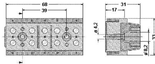
Dimensioned drawing
