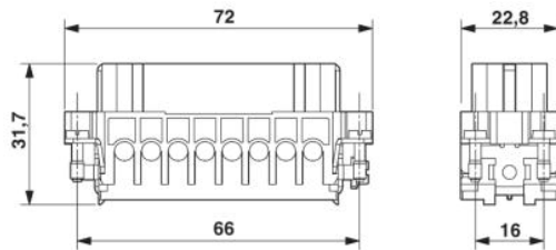
Female insert
