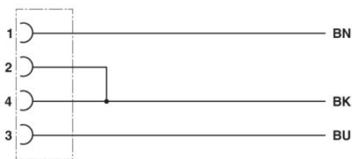
Contact assignment of M12 sockets bridged
