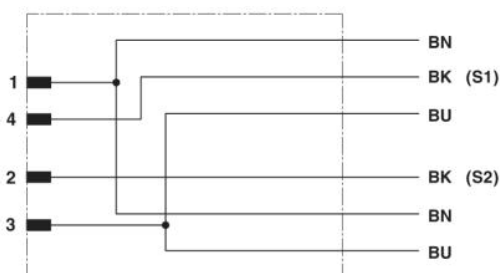
Contact assignment of the M12 Y plug connector
