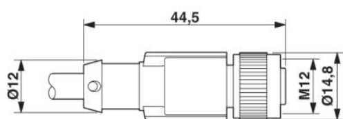
Socket M12 x 1, straight, with LED
