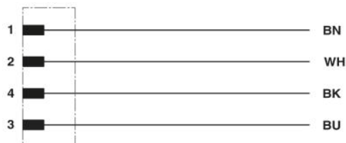
Contact assignment of the M12 plug
