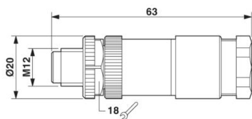
M12 x 1 male connector, straight
