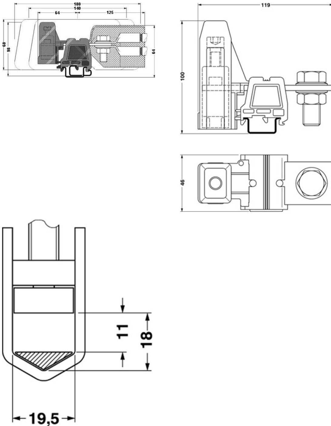
Dimensioned drawing
