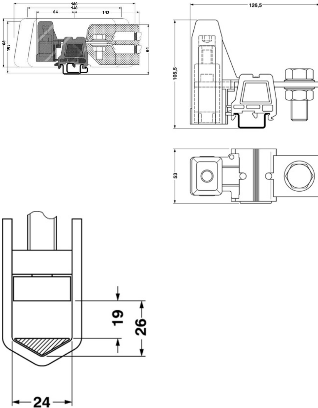
Dimensioned drawing
