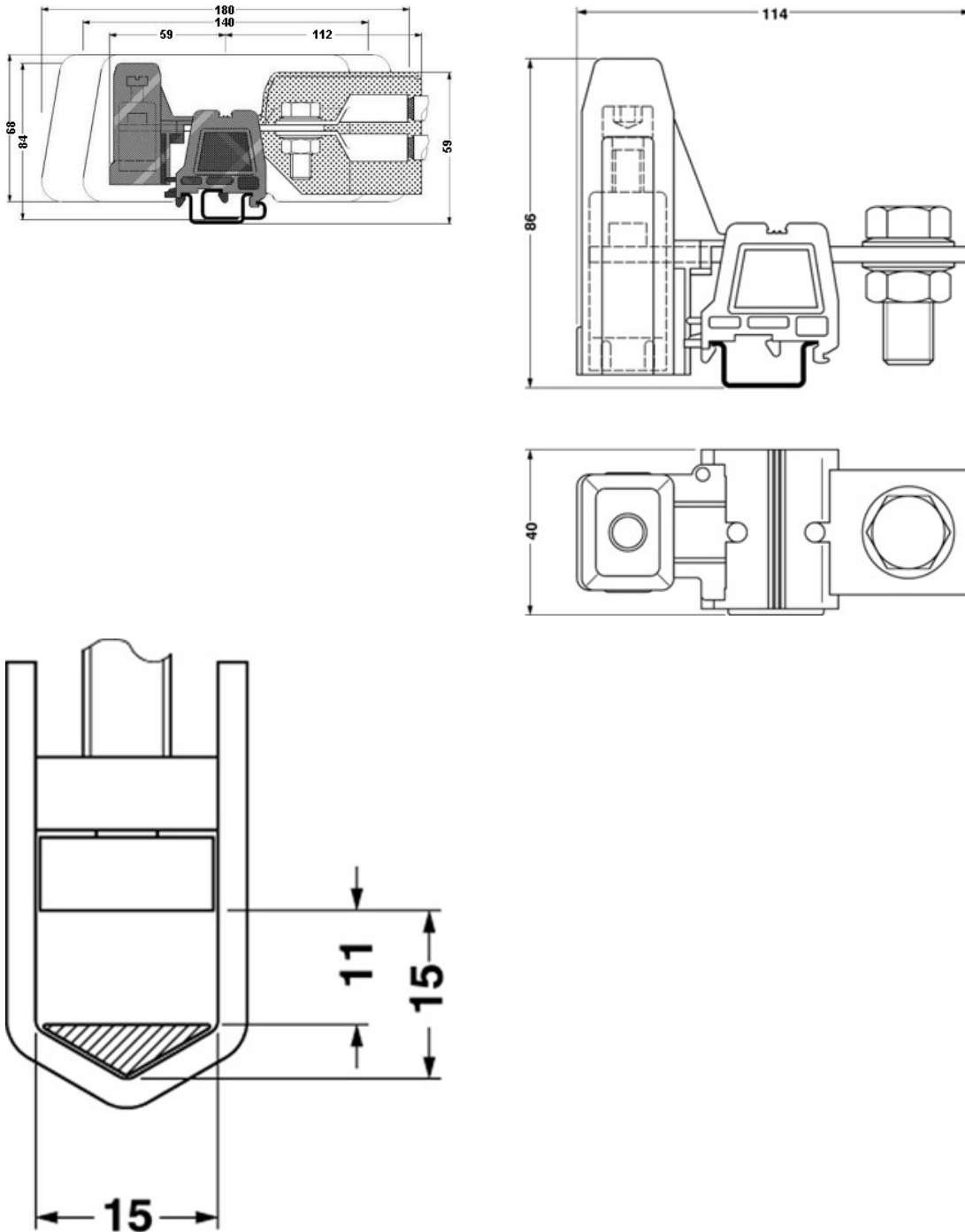
Dimensioned drawing
